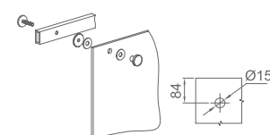
Guide Rail Installation Diagram
